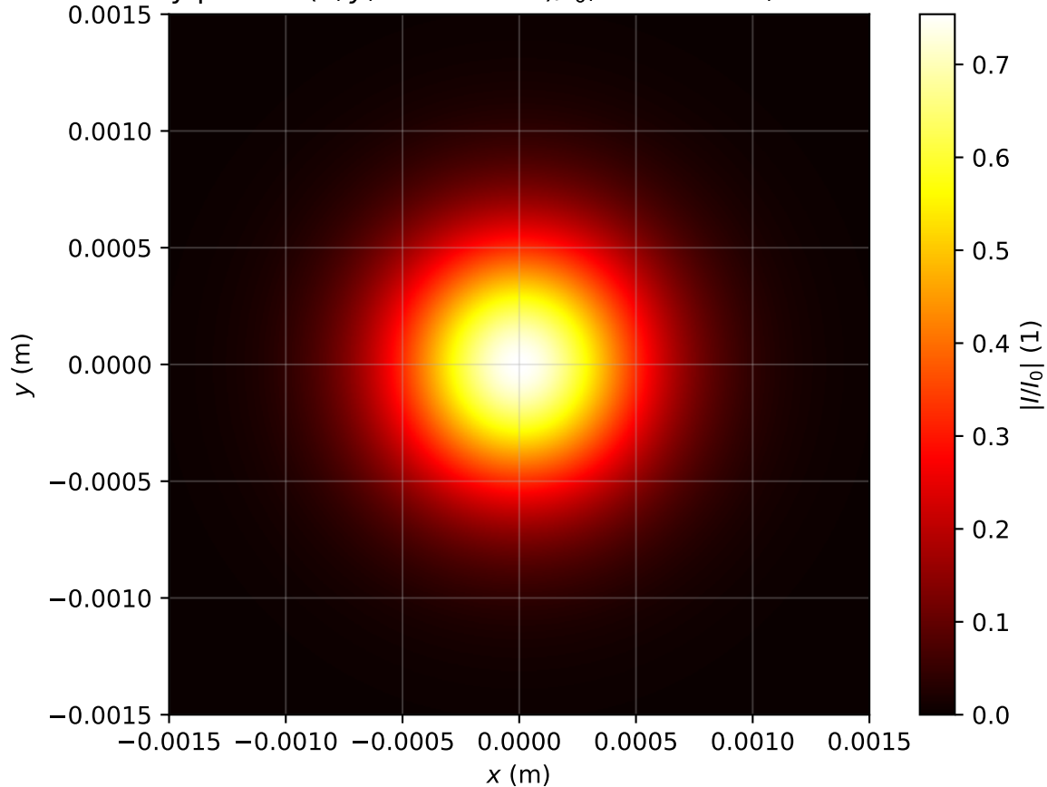
Intensity profile I(x, y, z = 1.911m)/I_0 , P_{in}=0.4P_{cr} , artificial time
